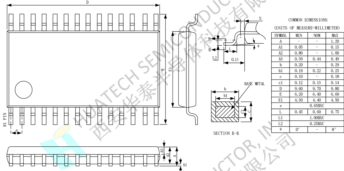
28-Lead TSSOP Package Outline Diagram
